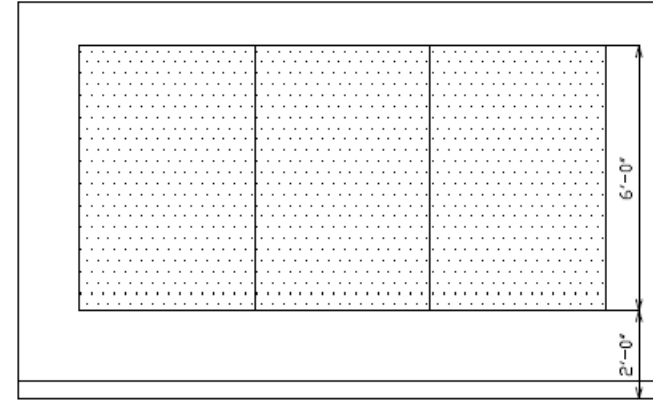
RM 156 – (3) 6'x4' WALL2WALL GLASSBOARDS CENTERED ON WALL
